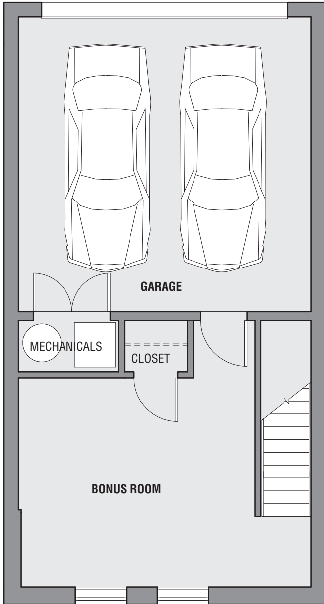
LEVEL ONE - ENTRY
